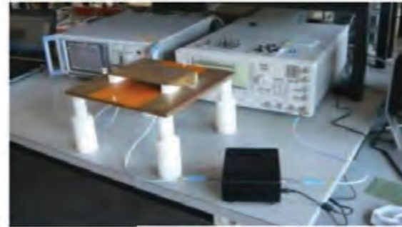
Stripline Fixture
