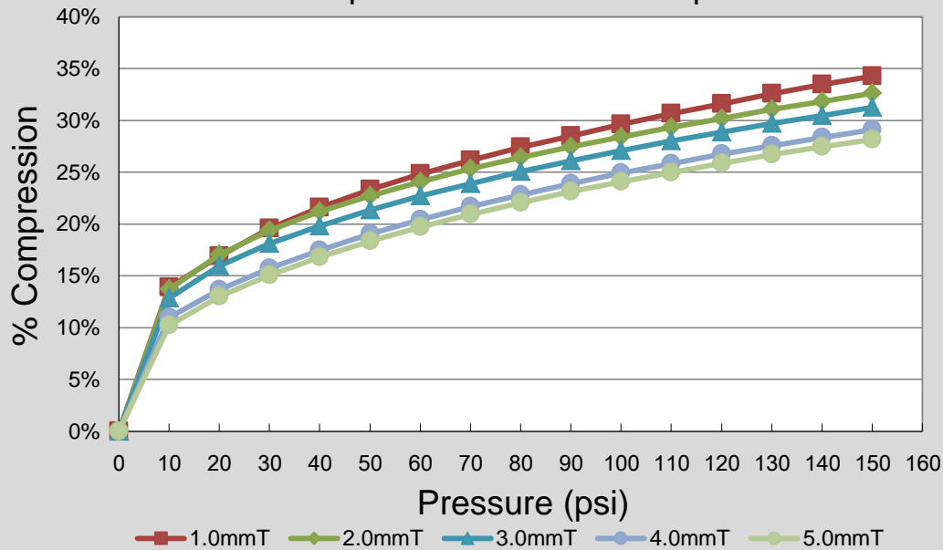
% Compression of OP-9400 Spec02
