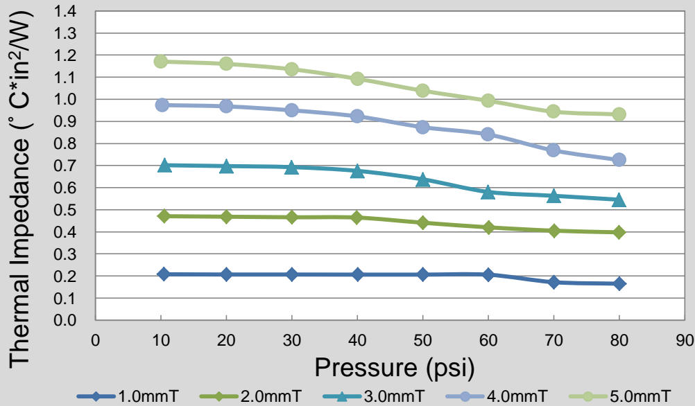
Thermal Impedance of OP-9400 Spec02
